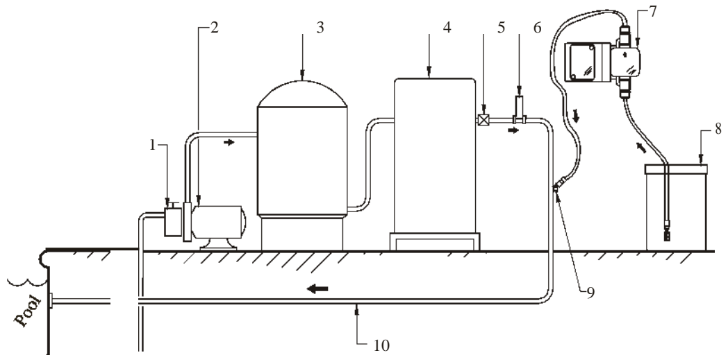
SWIMMING POOL INSTALLATION
