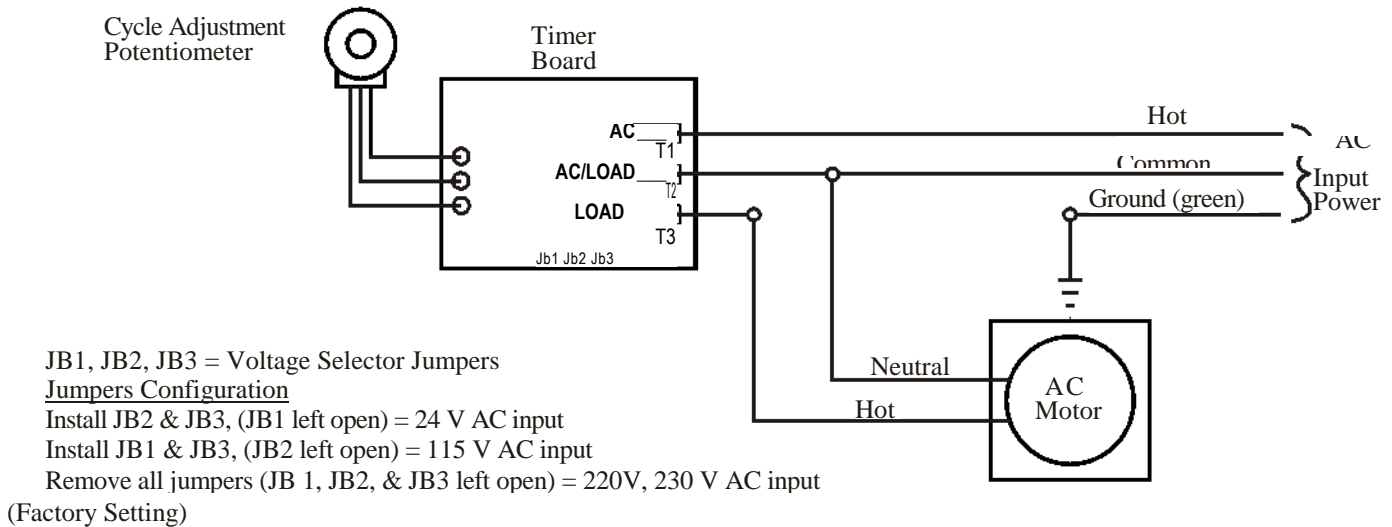
FIG. 4.6 WIRING DIAGRAM - FIXED TIMERS 4.3 How To Install
