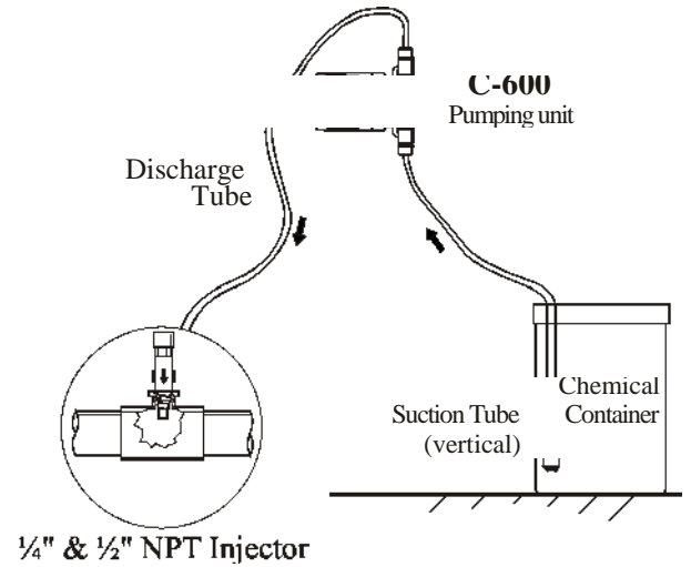
FIG. 4.2 TYPICAL INSTALLATION
