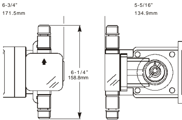
FIG. 4.1 DIMENSIONAL DRAWING
