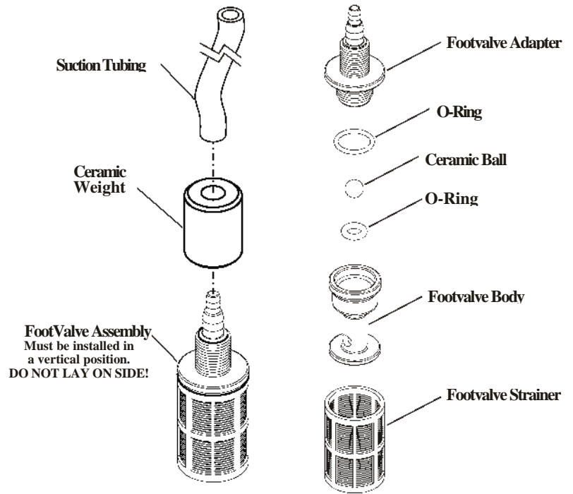
FIG. 4.8 FOOTVALVE ASSY.
